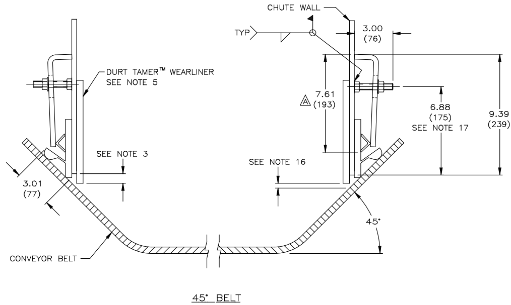
45° BELT
